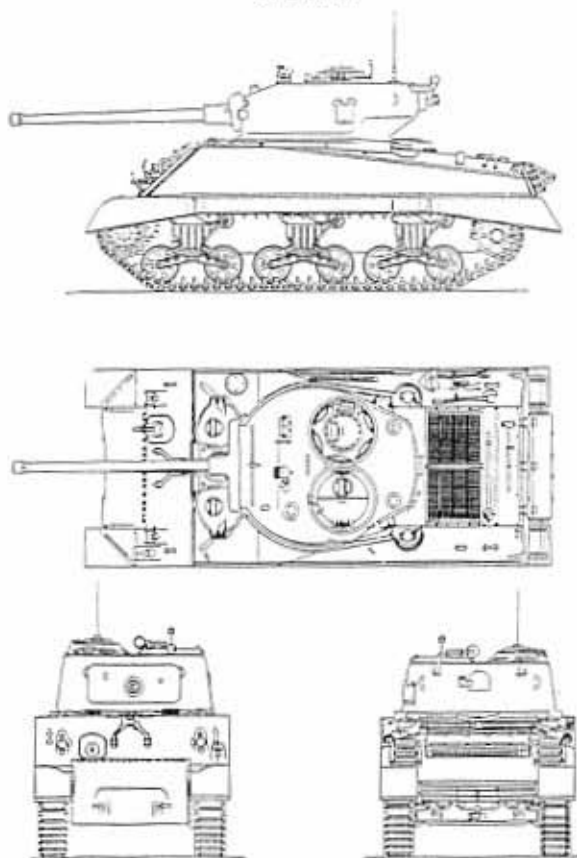
MEDIUM TANK M4A3 (76) W "SHERMAN"
